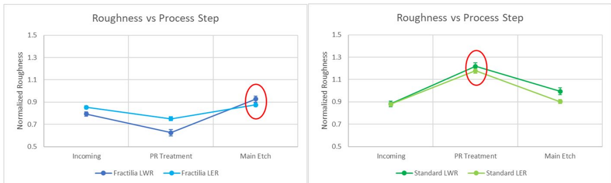
Figure 13 (left): Fractilia LWR and LER as a function of process step
